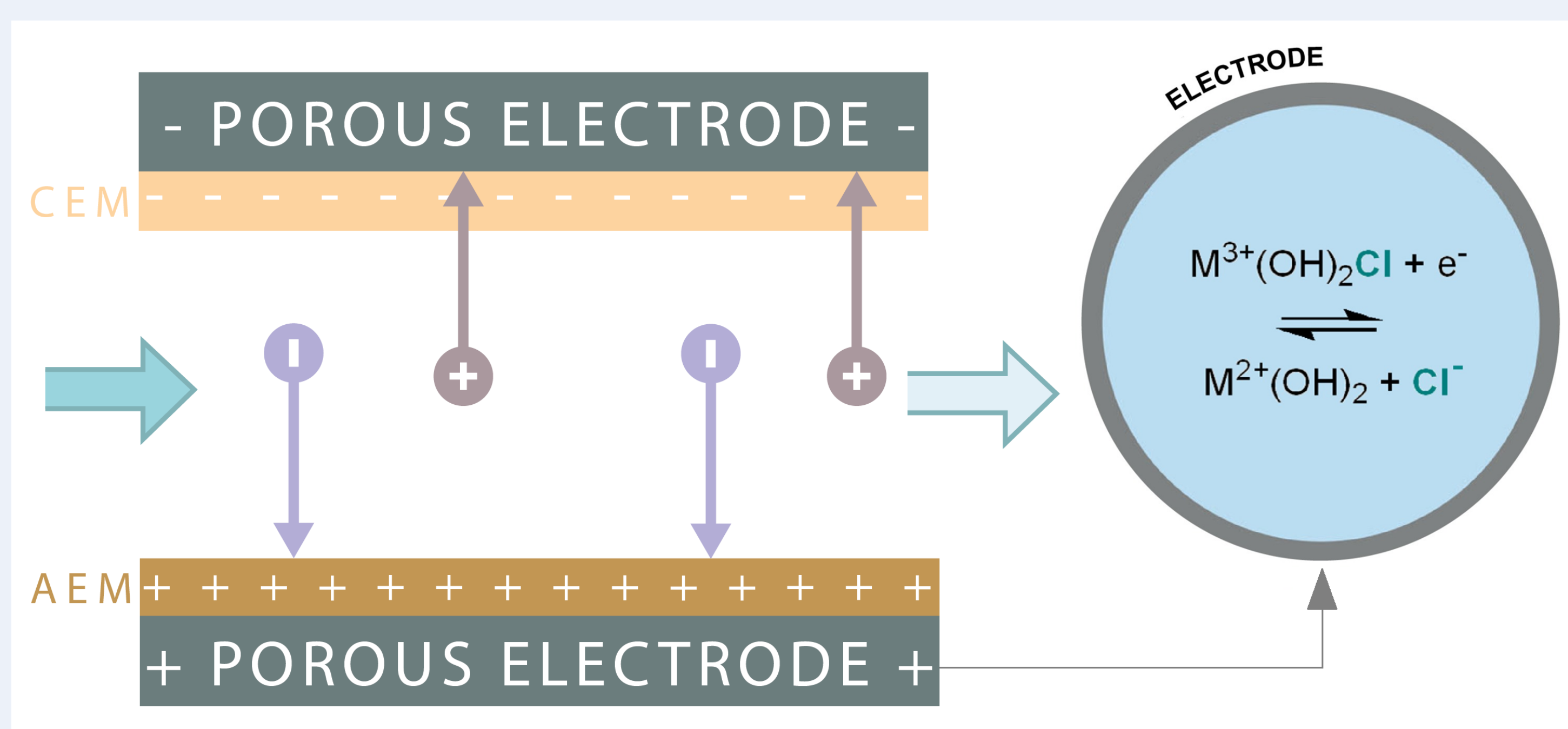
Fig.2 Schematic design of a cell for Membrane Capacitive Deionization (MCDI); in the outer circle is represent the exemplary and generalized mechanism of the electro-adsorb ions materials that will be studied.
