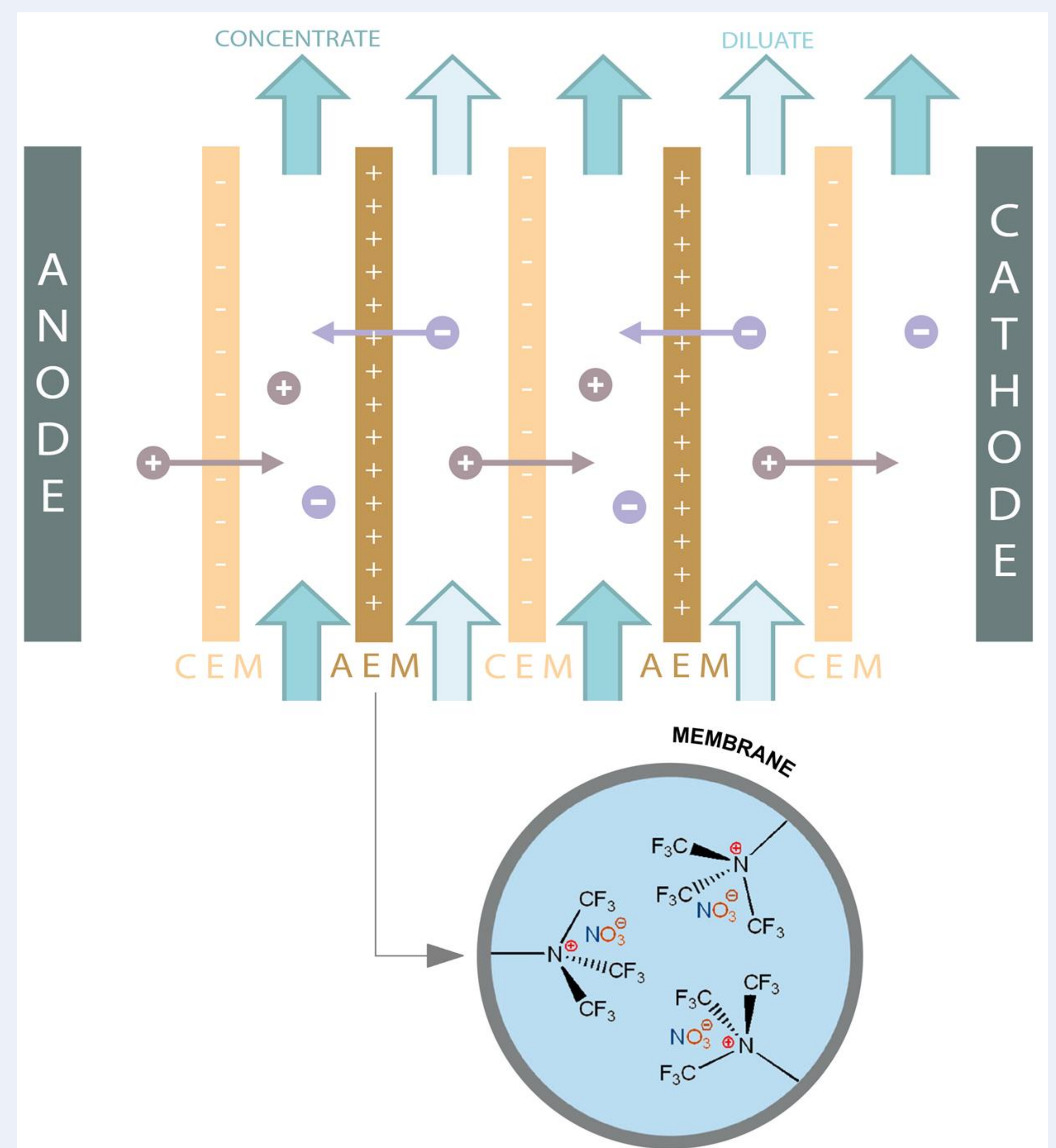
Fig.1 Scheme of an electro dialysis system, identifying the repeating unit (cell pair); in the outer circle is represent the exemplary and generalized structure of the ion-exchange polymer membranes that will be studied.
