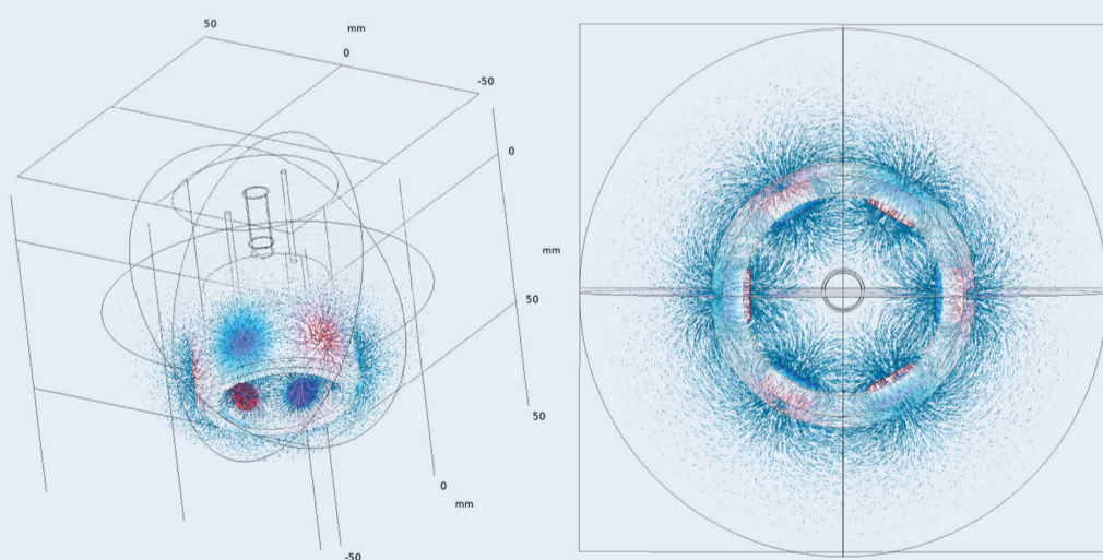
Fig. 2. Schematic of a rotating magnetic field with alternatively oriented north-south (N-S) configuration for nano bubble stabilisation
