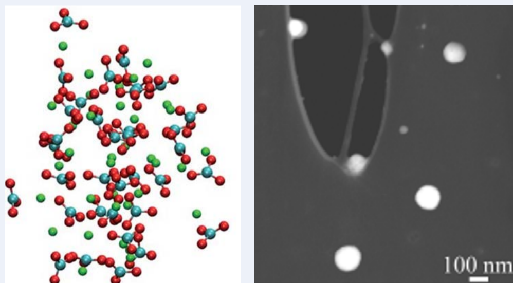
Fig 1. a) Snapshot of amorphous calcium carbonate nanoparticles taken from molecular dynamics simulation (left) [2] and b) TEM (right) (white spheres) [3].
