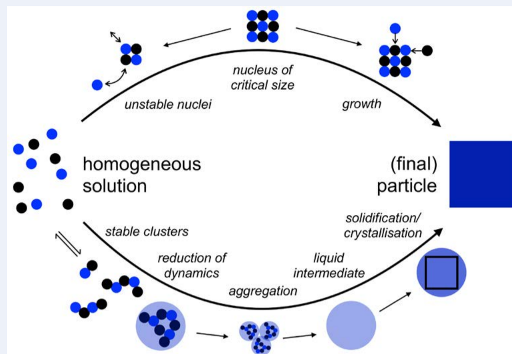
Fig. 2 Schematic illustration of the mechanism of nucleation of DOLLOPs according to classical nucleation theory (CNT, top) and the pre-nucleation cluster (PNC) pathway (bottom) [8]. The PNC pathway has gained more attentions during the last years and it can be more rationalized for creating DOLLOPs in \text{CaCO}_3 solutions in different experiments.
