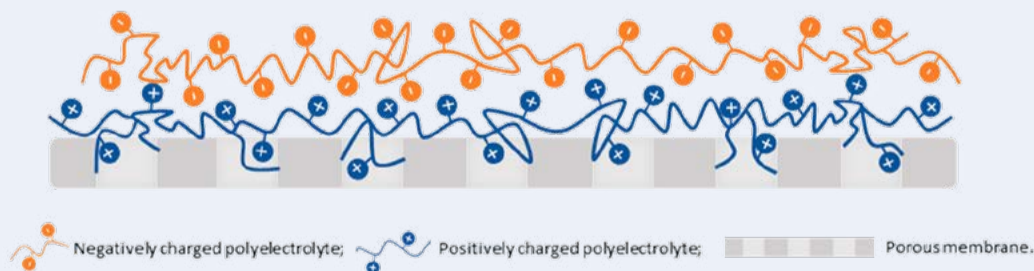
Fig 1. Schematic illustration of a low fouling NF membrane prepared by polyelectrolyte layer-by-layer deposition on ultrafiltration membrane.
