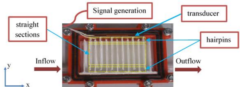
Figure 1 – The novel serpentine separator prototype
